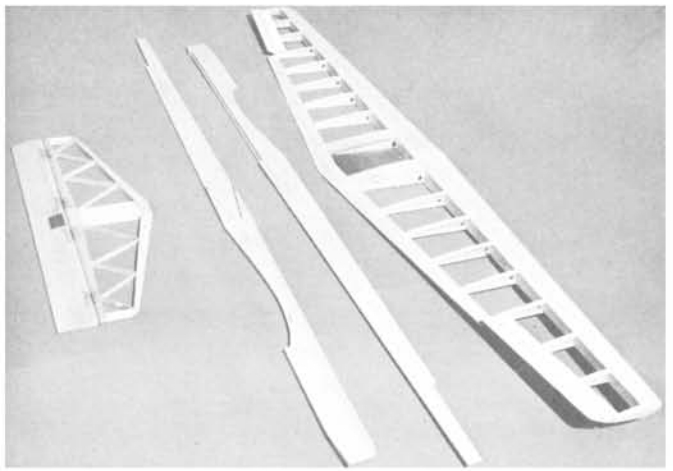
Skydancer is built like any model plane, but it must be stronger to withstand acceleration and high speed in launch.
